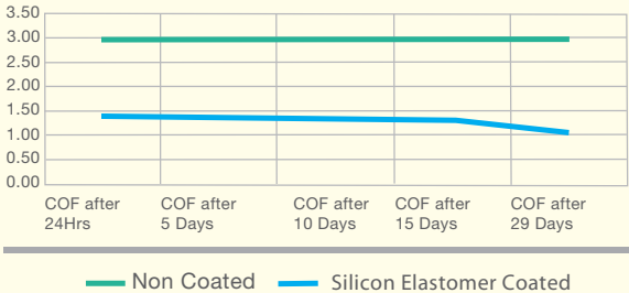
Change in Coefficient of Friction over time
